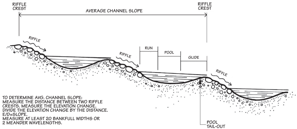
Stream profile
