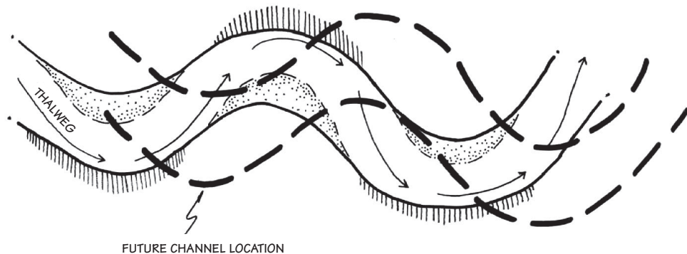
Channel migration
